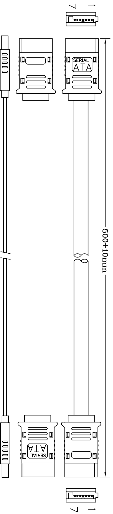
SERIAL ATA 7P (BLACK ASS'Y)
