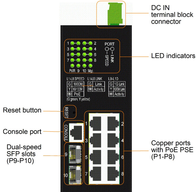
Front panel
