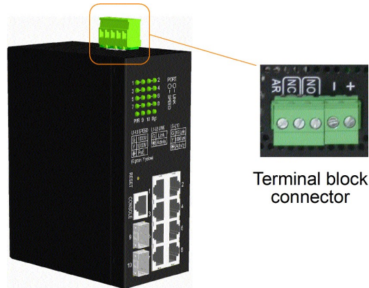
Top panel
